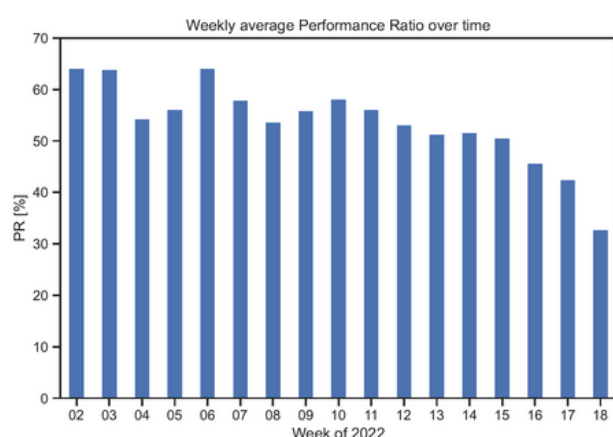
Figure 2: Weekly average performance ratio (PR) for the system. The gradual reduction indicates that the system is undergoing degradation outdoors.
